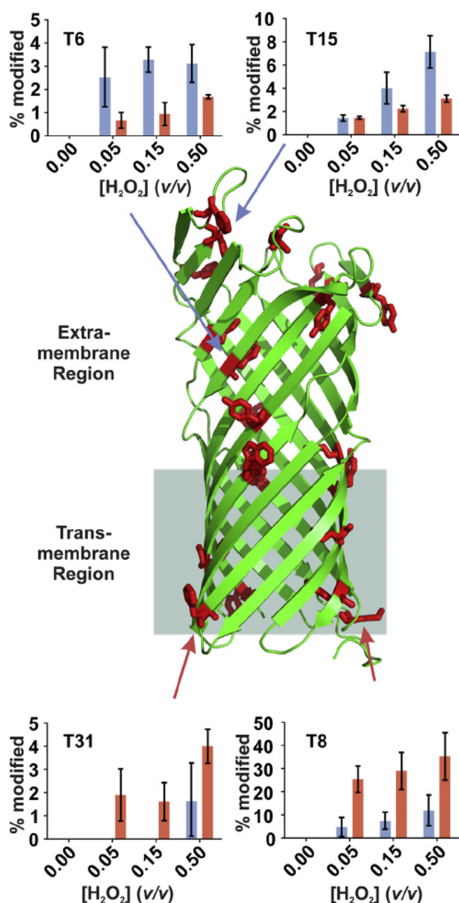
Fig. 9. FPOP-MS analysis of OmpT solubilized in either DDM detergent micelles or amphipol A8-35. Graphs show the % modified of four peptides in DDM (blue) or amphipol (orange). Arrows show the residues modified in each case. Residues in the extra-membrane region are more readily labelled in DDM, whilst residues at the lower boundary of the transmembrane region are more readily labeled in amphipol. Figure is reproduced from Ref. [218]. (For interpretation of the references to color in this figure legend, the reader is referred to the web version of this article.)
